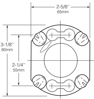
Intermediate Flange
