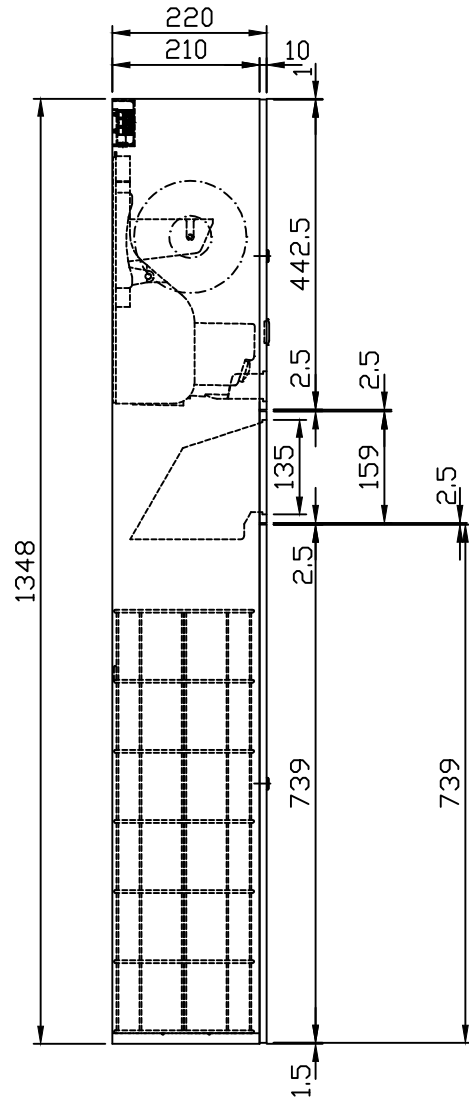
Detail X
